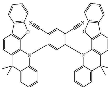
[chemical formula 7]
