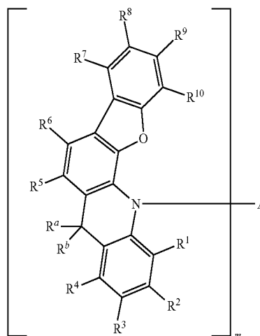
[chemical formula 1]
