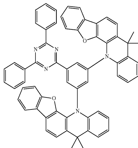
[chemical formula 10]
