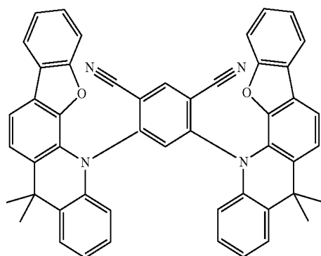
[chemical formula 7]
