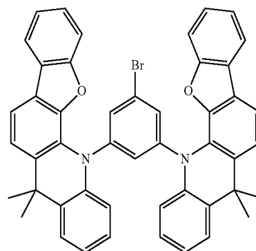
[chemical formula 9]
