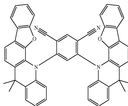
[chemical formula 8]
