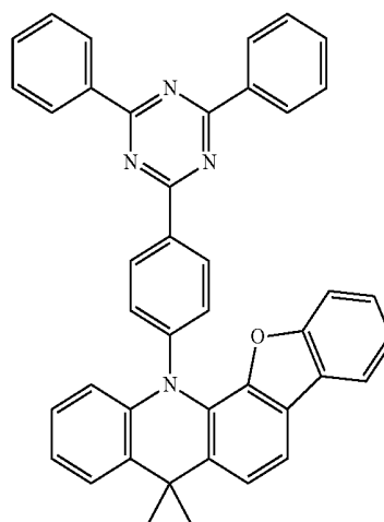
[chemical formula 5]
